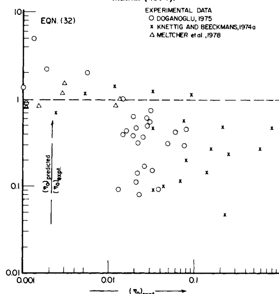
Figure 7. Comparison of experimental data with correlation by Meltcher et al. (1978).
