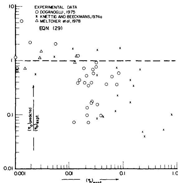
Figure 5. Comparison of experimental data with correlation by Paretzky (1972).
