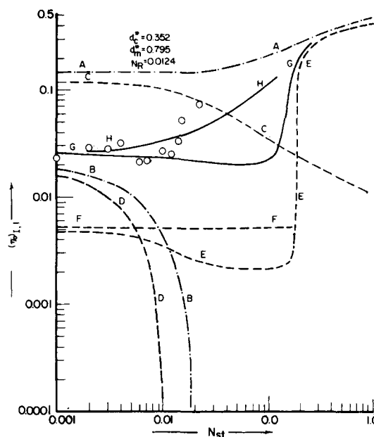
Figure 4a. Variation of (\eta_0) with N_{St}, N_R = 0.0124 .
