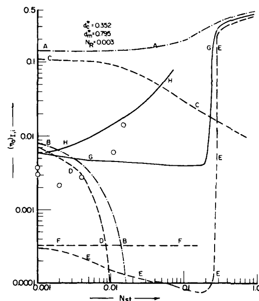
Figure 4b. Variation of (\eta_0) with N_{St}, N_R = 0.003 .
